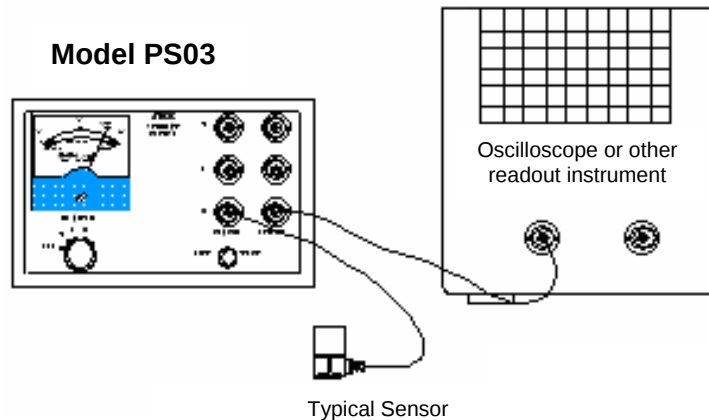
Figure 2. Systems Interconnect
