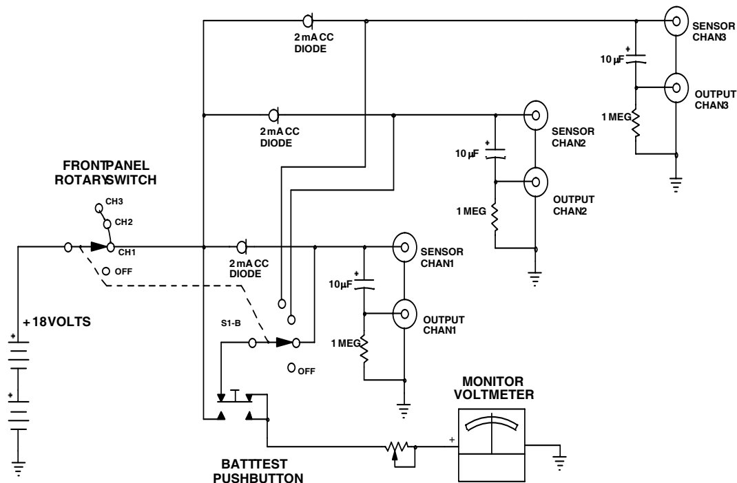
Figure 1. Schematic Diagram, PS03
